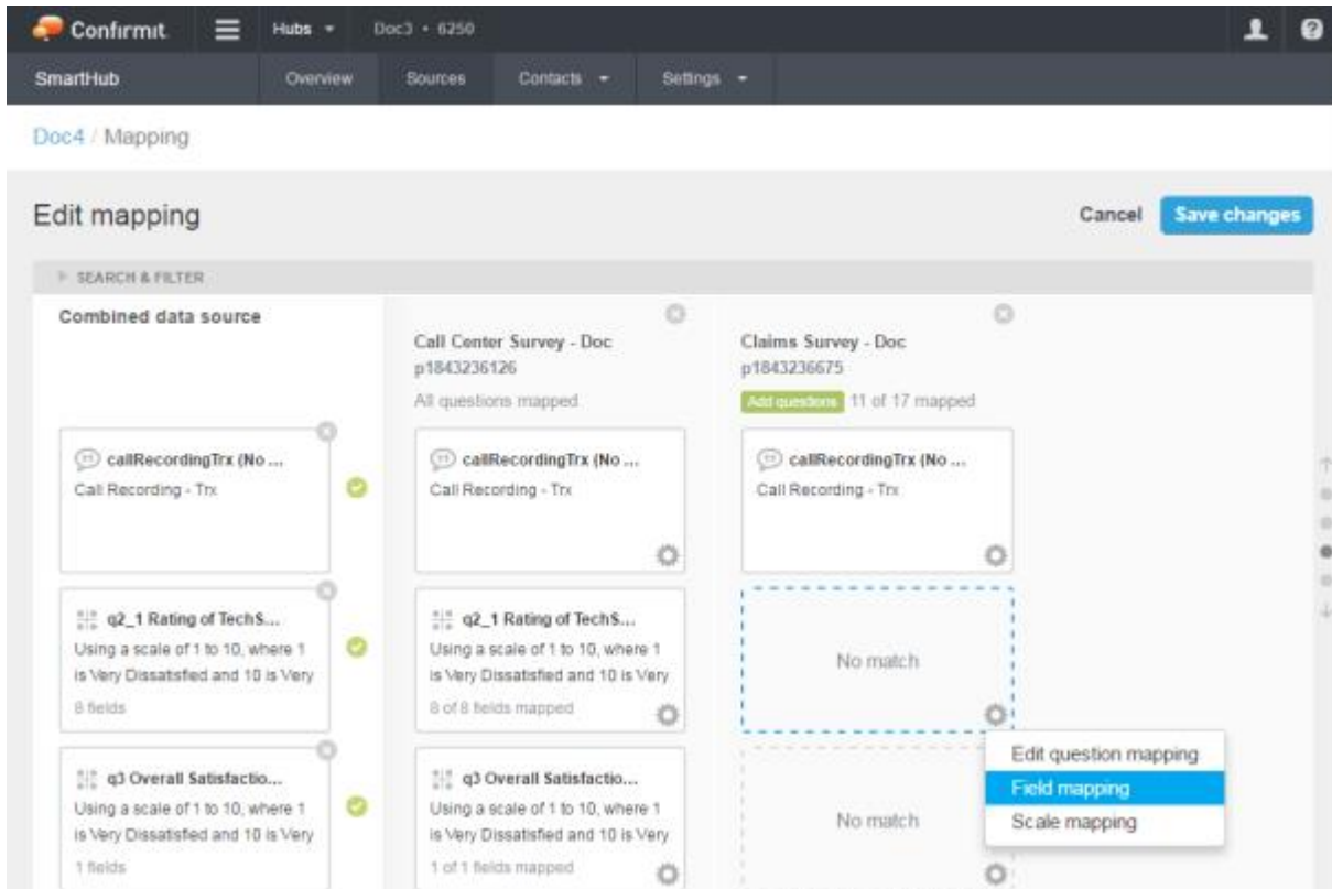
Figure 49 Selecting Field mapping for a grid question
