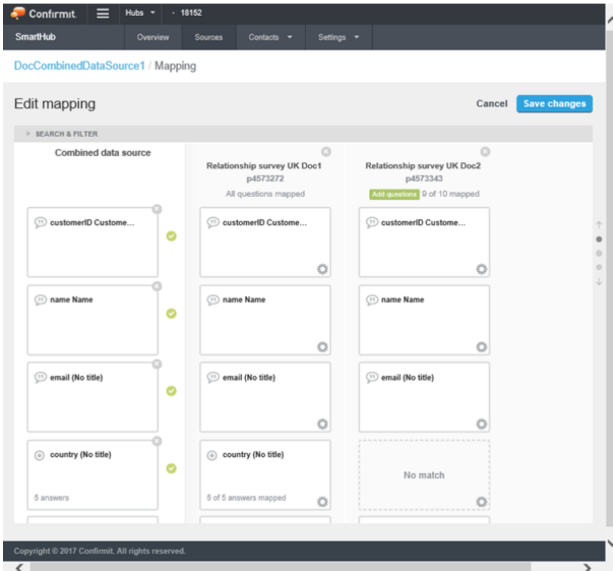
Figure 30 Example of the Edit mapping page for a combined data source
