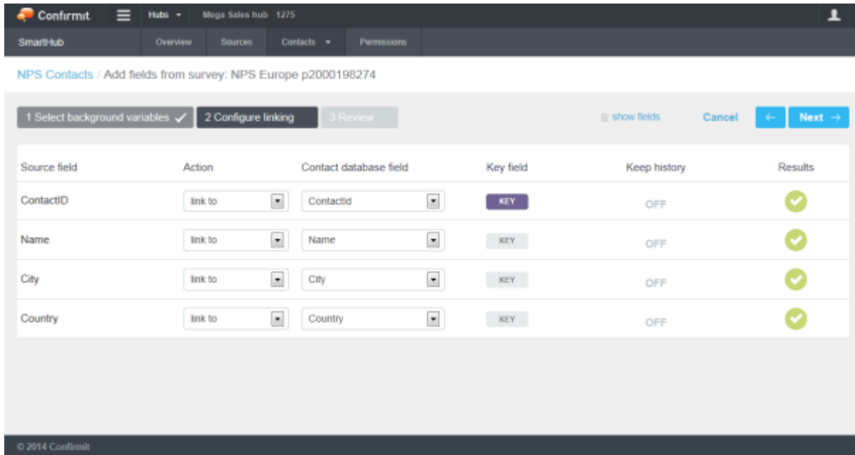
Figure 80 Example of the Configure linking page
